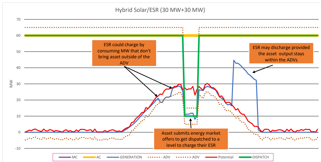
Figure 1 – Energy offers that permit charging of the energy storage component of a source asset
