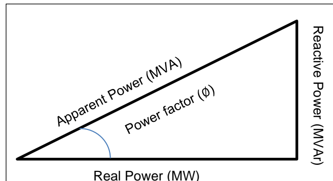
Figure 1: Power Triangle
