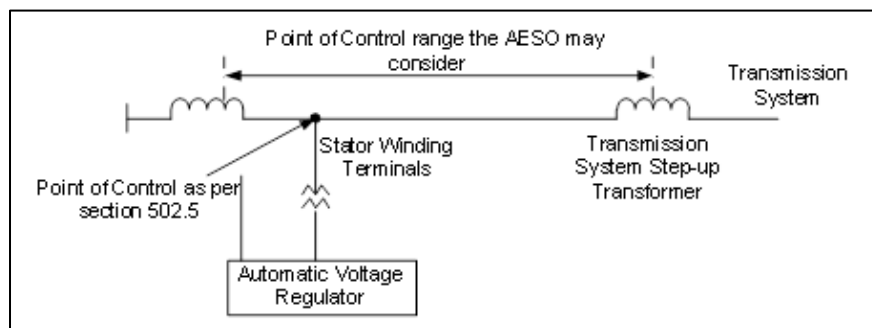
Figure 3: Point of Control, Simplified Impedance Diagram of a Single Generating Unit
