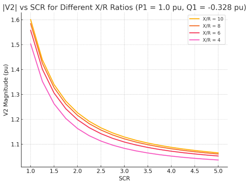
Figure 8: |V_2| vs SCR for Different X/R Ratios ( P_1 = 1.0\text{pu} , Q_1 = -0.328\text{pu} )
