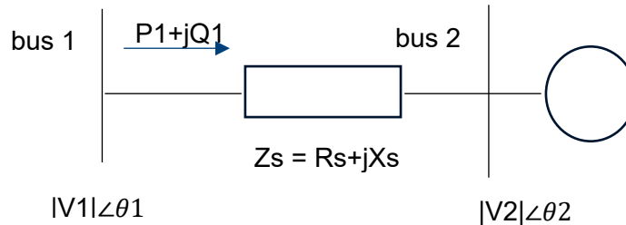
Figure 9: The Equivalent System
