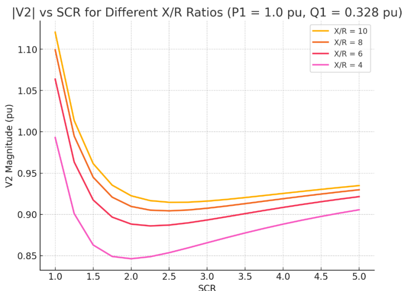
Figure 7: |V_2| vs SCR for Different X/R Ratios ( P_1 = 1.0\text{pu} , Q_1 = 0.328\text{pu} )
