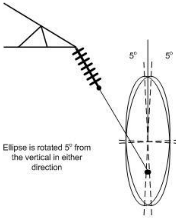
Galloping Envelope
