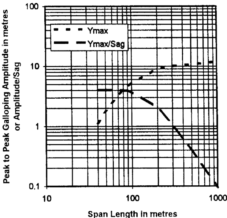
Figure 2 Observed Galloping Amplitude vs. Span Length
