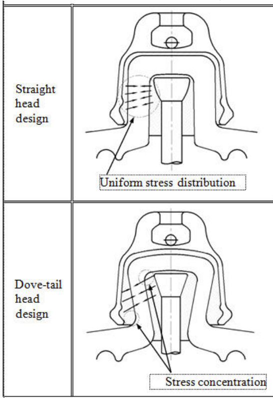
Figure 1 Insulator Head Designs
