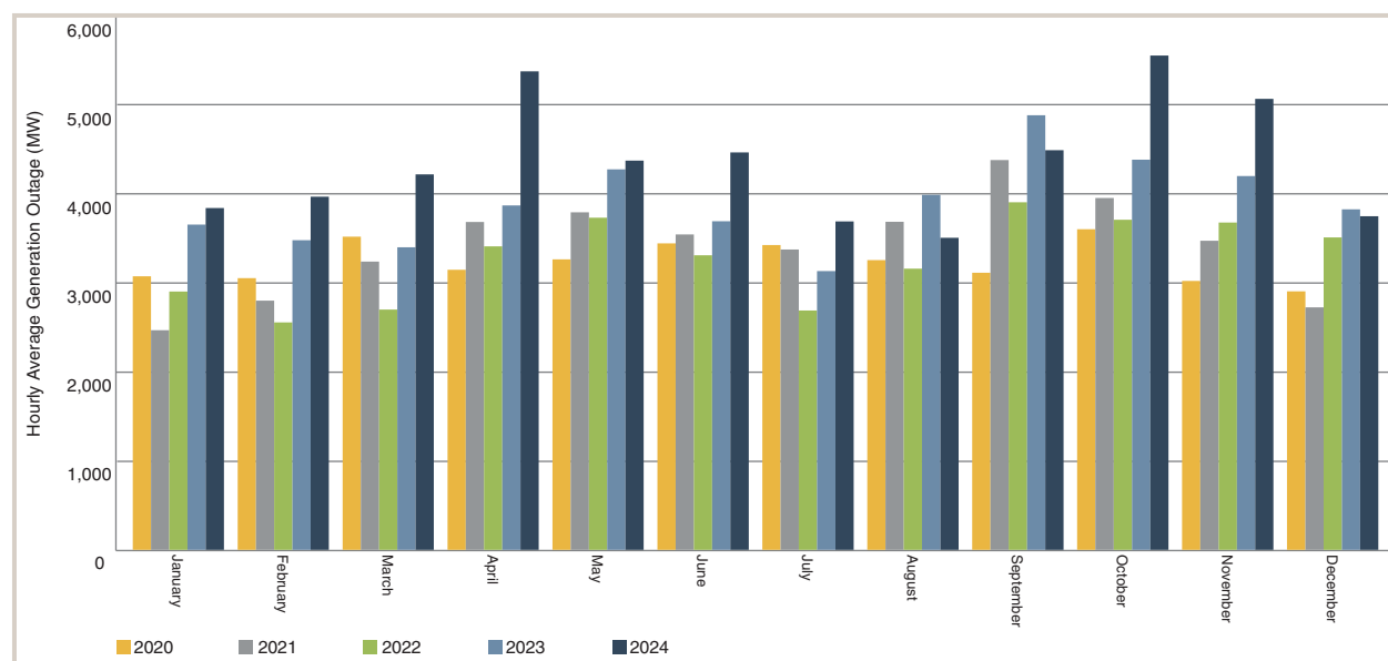
FIGURE 36: Generation Outages by Month
