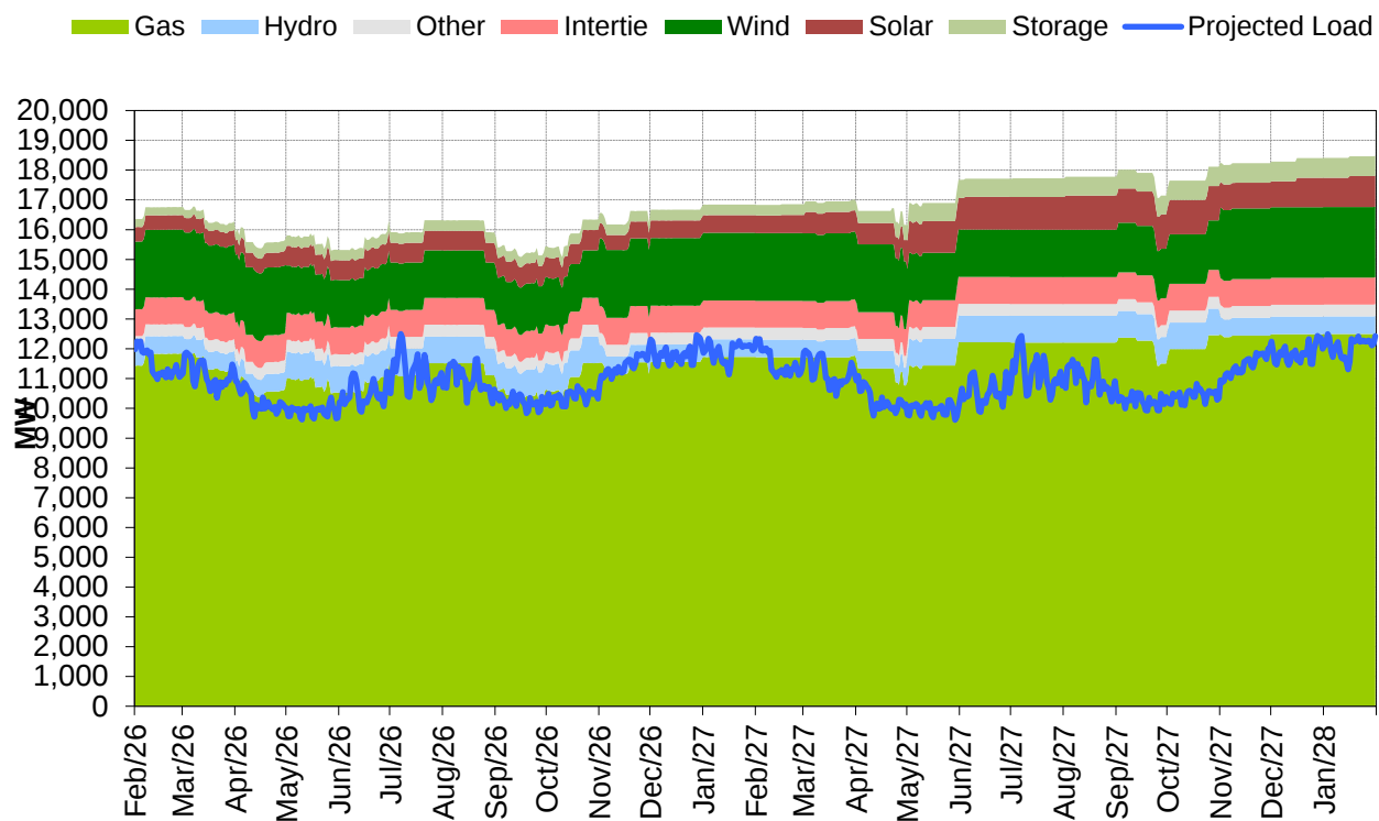
Figure 3: Alberta Internal Load (AIL) Daily Peak Demand and Available Supply February 1, 2026, to January 31, 2028
